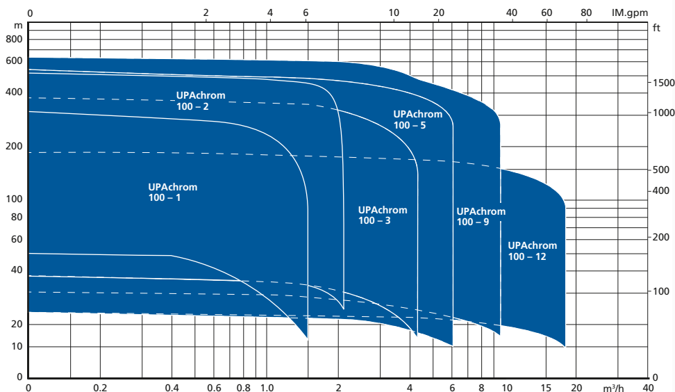
Characteristic curves UPAchrom 100CC (50 Hz)
