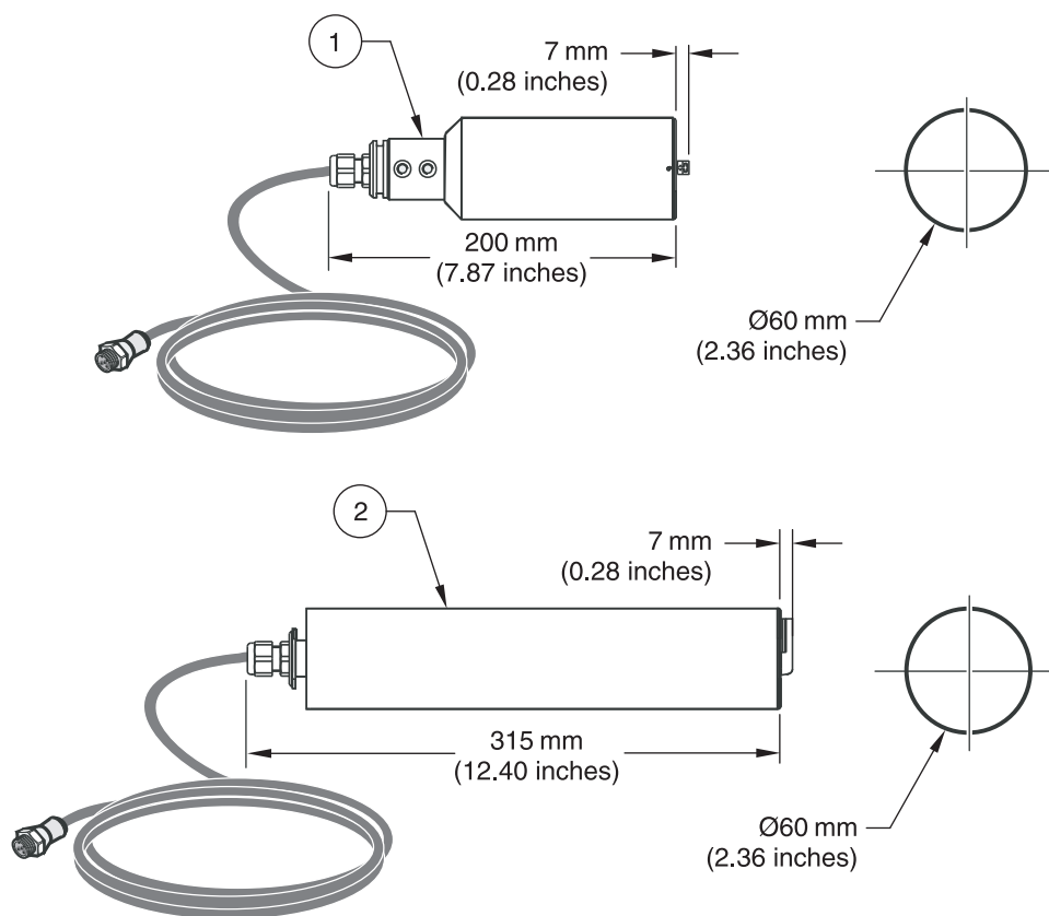
Figure 1 Sensor Dimensions
