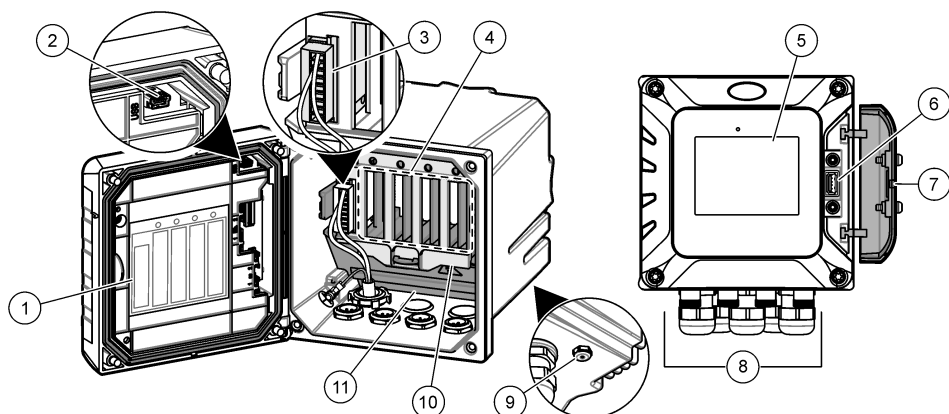
Figure 1 Product overview
