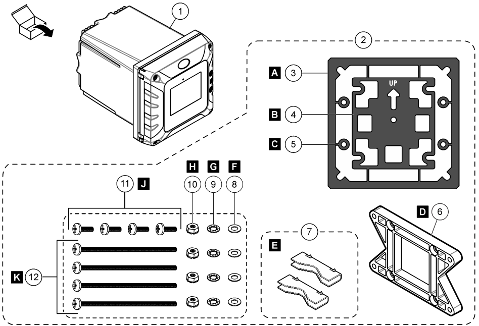
Figure 2 Product components
