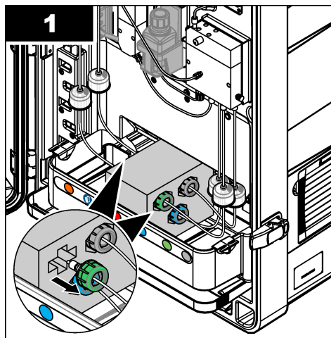
Figure 14 Chemical installation
