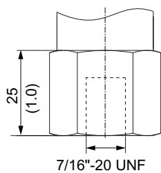
Figure 9-3 Max. 20 Nm
